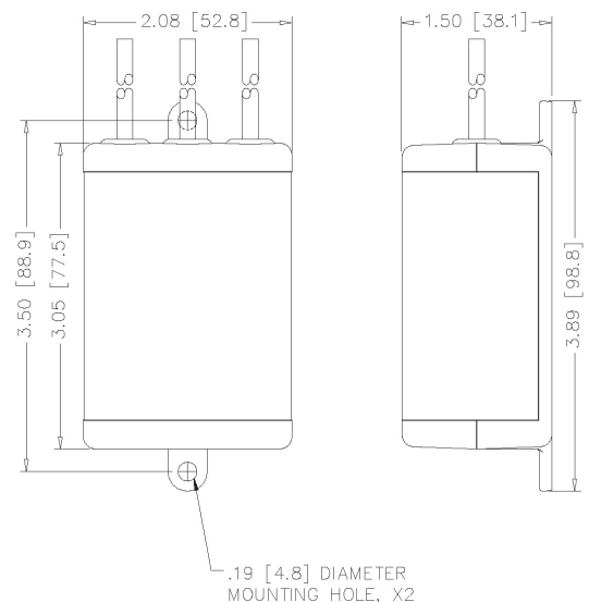
Figure 2: - LS12N models
