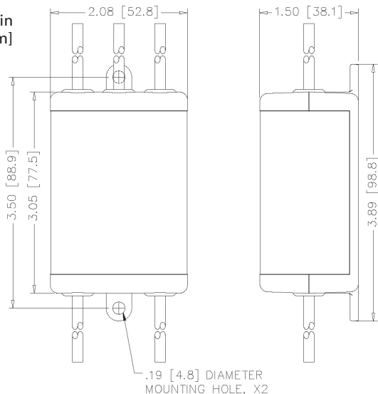
Figure 1: - LS10N models
